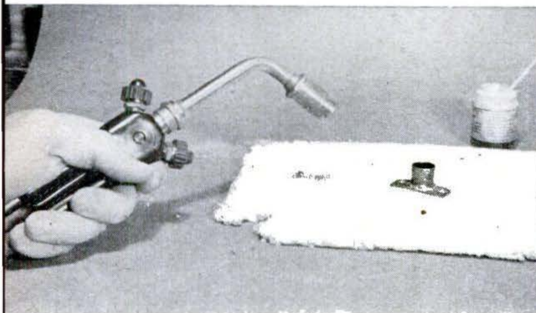
COOKING GAS , boosted with compressed air, produces a hot, clean flame suitable for silver soldering and brazing.
